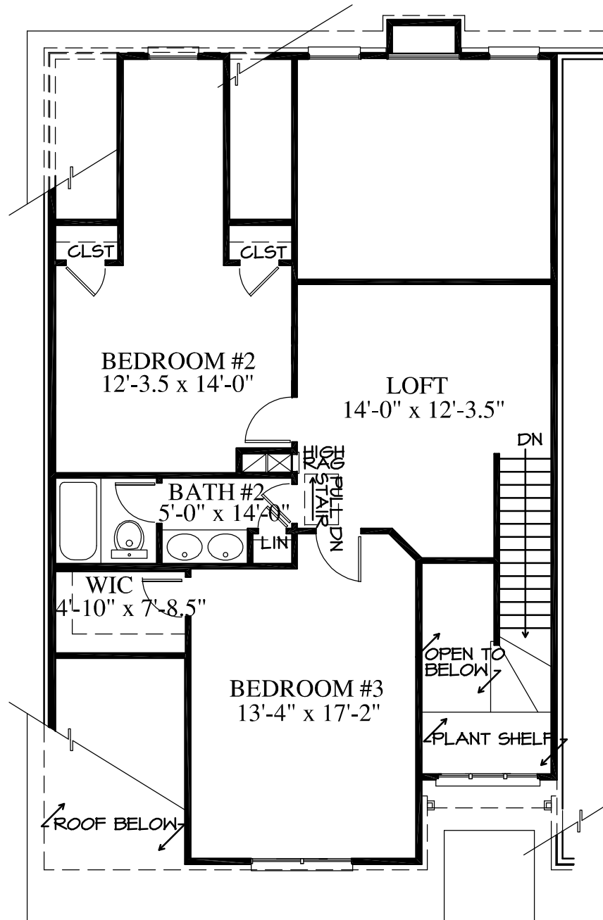
UNIT D UPPER FLOOR PLAN
